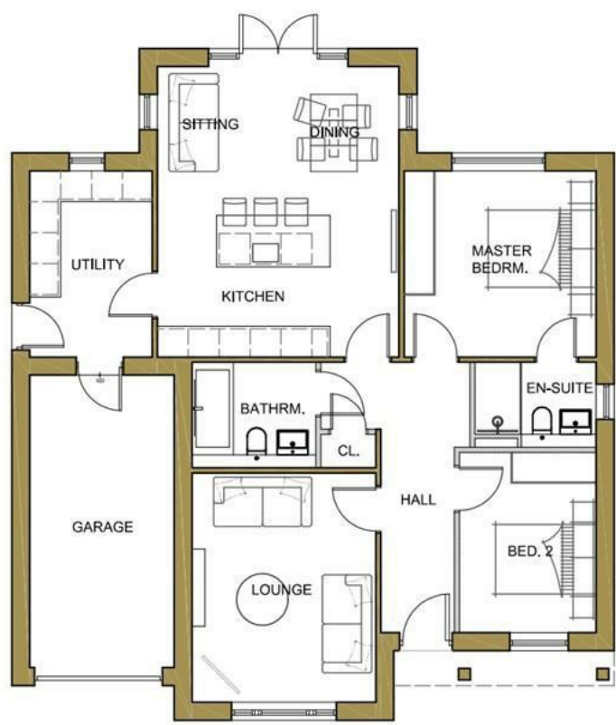
FLOOR PLAN
